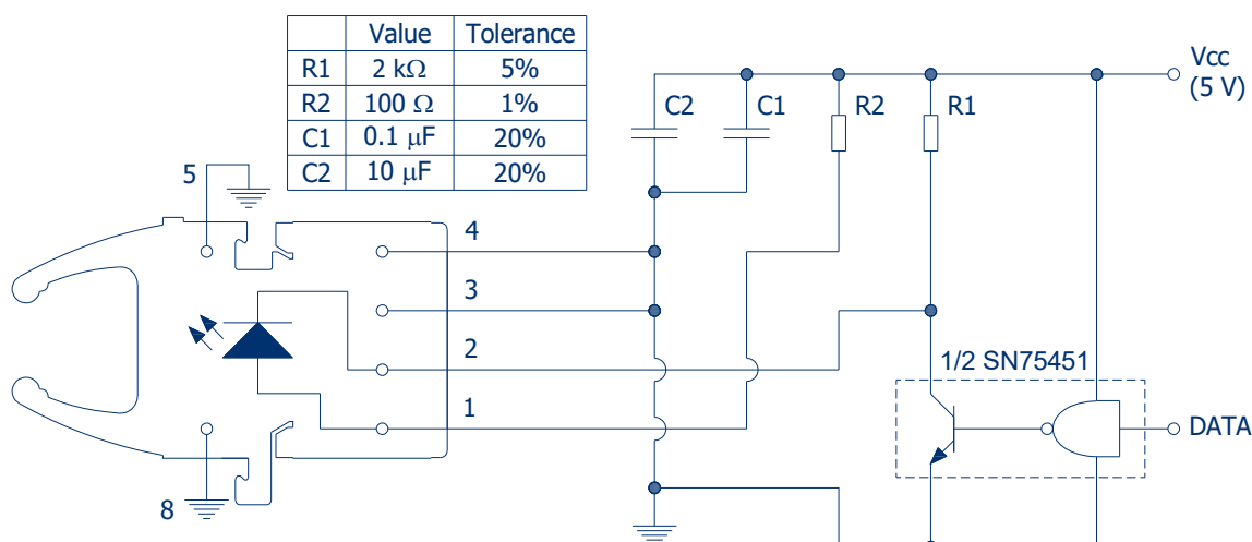
FIGURE 2 Recommended transmitter application circuit. See note 6, Table 6
