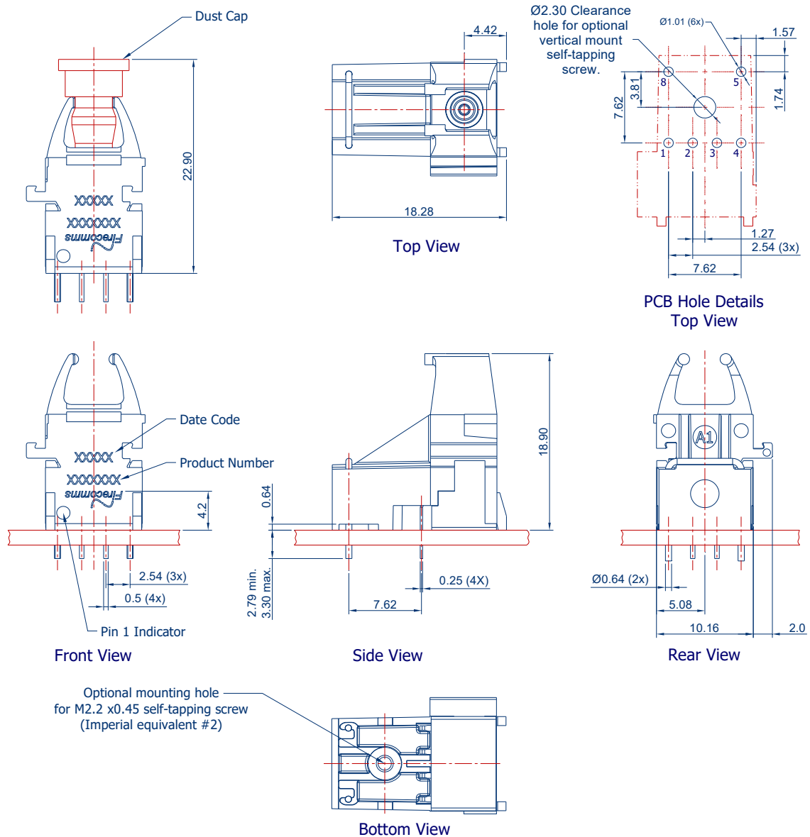
FIGURE 8 Mechanical dimensions of RedLink® vertical connectors and PCB footprint, which is a top view General dimensional tolerance is ± 0.2 mm
