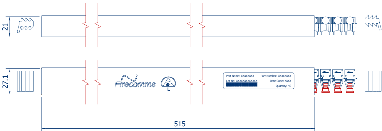
FIGURE 11 Packing tube for Firecomms RedLink® tilted connectors
