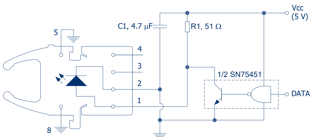
FIGURE 2 Recommended transmitter application circuit. See note 6, Table 6
