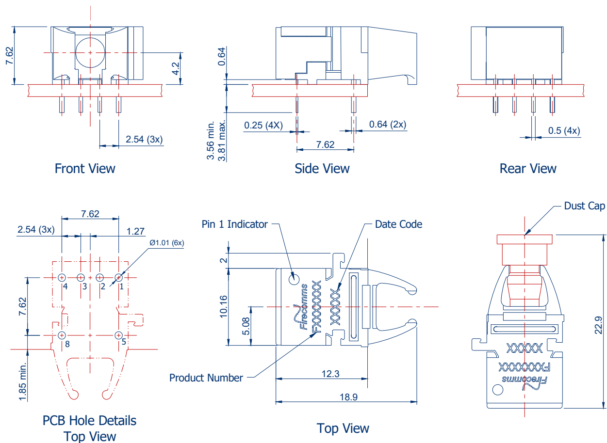
FIGURE 4 Mechanical dimensions of the horizontal receivers and PCB footprint, which is a top view General dimensional tolerance is \pm 0.2 mm
