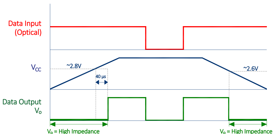
FIGURE 6 Non-inverting receiver output operation during power cycling
