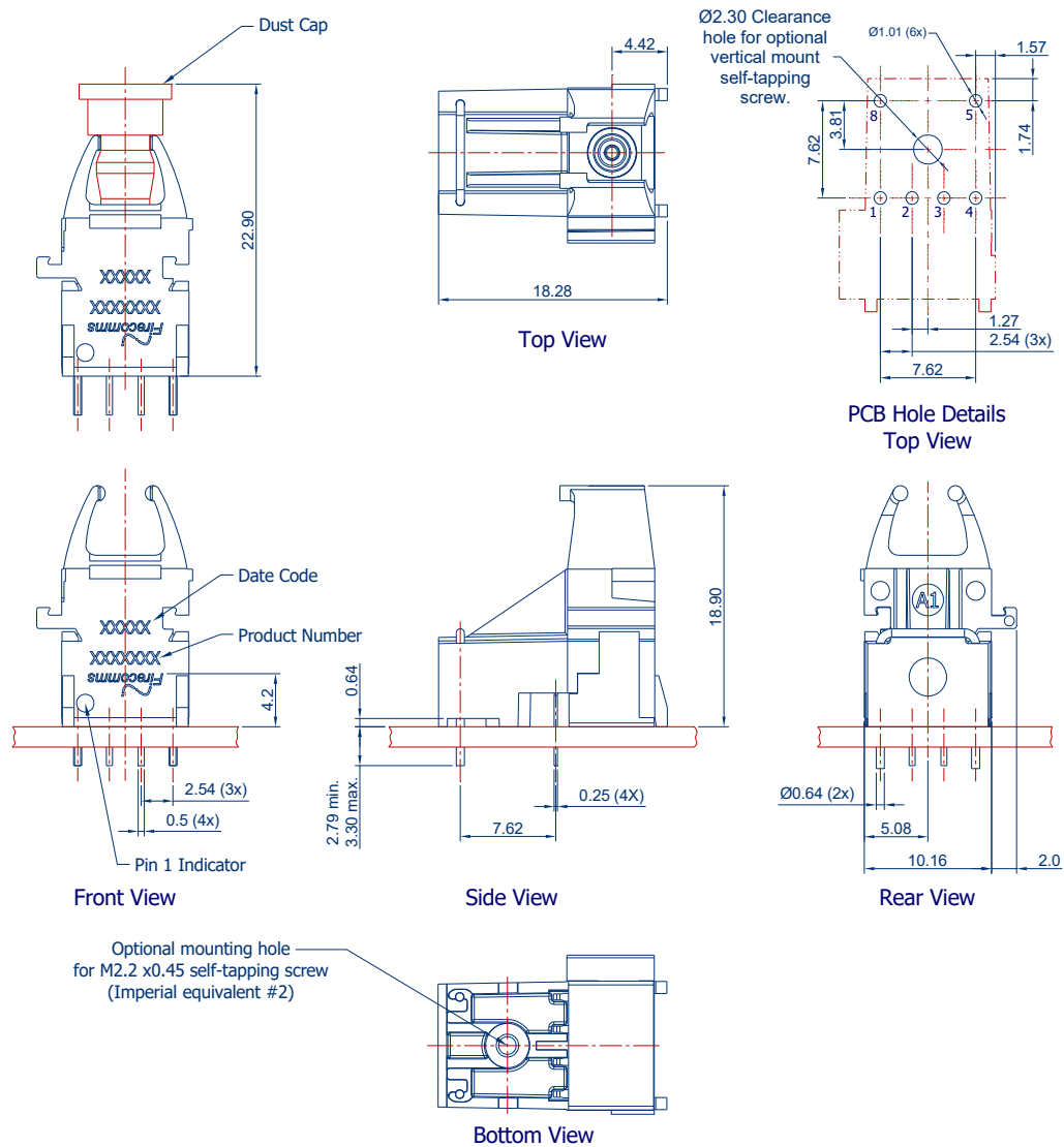
FIGURE 9 Mechanical dimensions of RedLink® vertical connectors and PCB footprint, which is a top view General dimensional tolerance is \pm 0.2 mm
