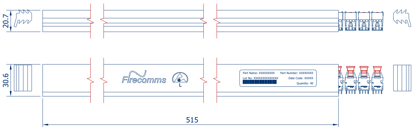
FIGURE 10 Packing tube for Firecomms RedLink® vertical connectors
