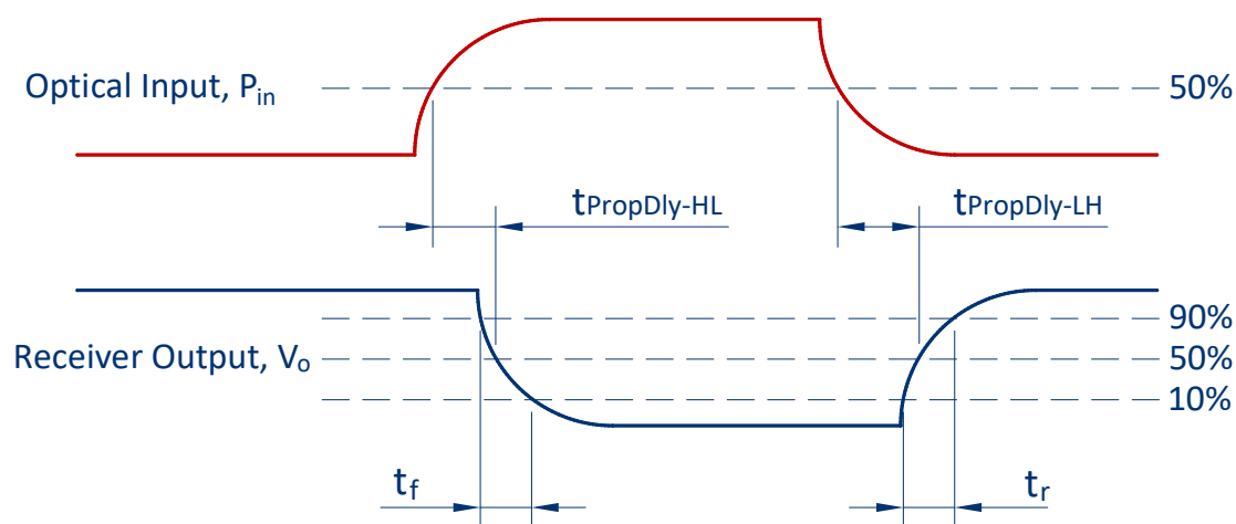
FIGURE 2 Receiver propagation delay and rise/fall time definitions
