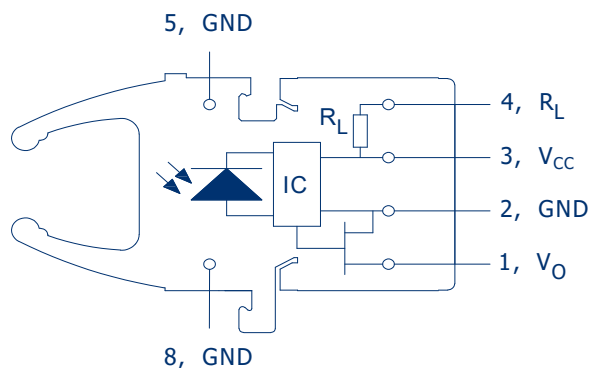
FIGURE 1 Receiver pin-out, top view
