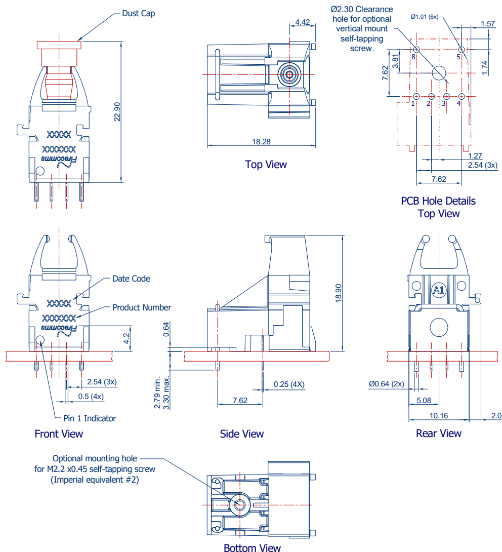
FIGURE 6 Mechanical dimensions of RedLink® vertical connectors and PCB footprint, which is a top view General dimensional tolerance is \pm 0.2 mm
