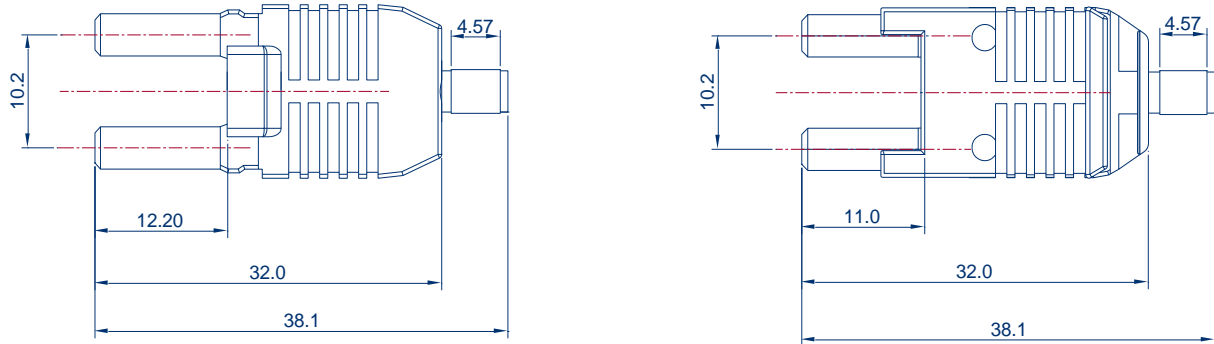
FIGURE 1. Duplex Non-Latching and Latching Plug mechanical dimensions
