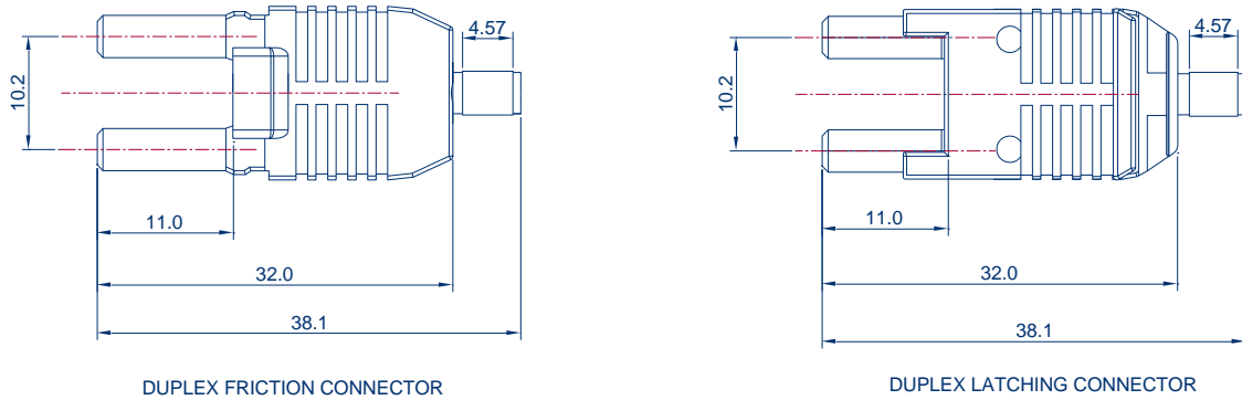
FIGURE 1. Duplex Non-Latching and Latching Plug mechanical dimensions
