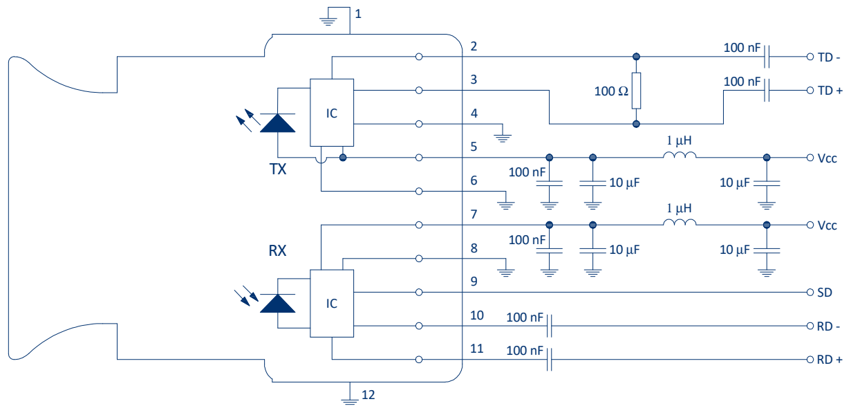
FIGURE 2 Recommended application circuit schematic to AC couple to a PHY
